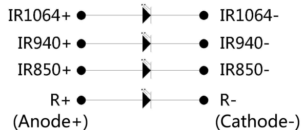
Circuit diagram
