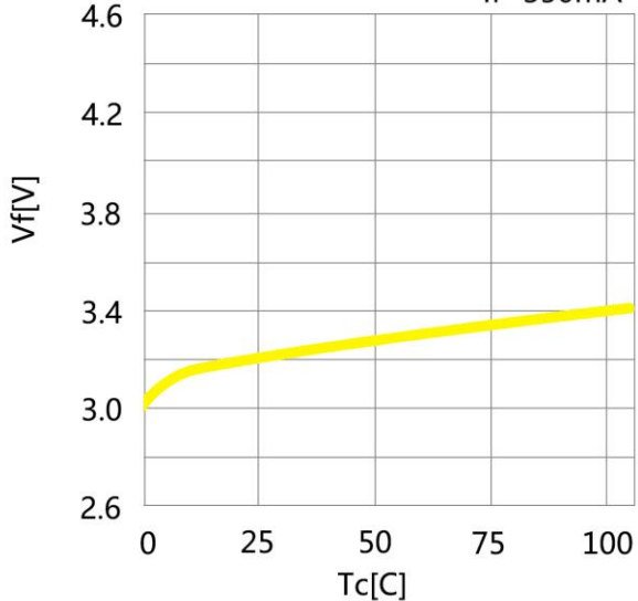
Case Temperature vs. Forward Voltage I_f=350\text{mA}
